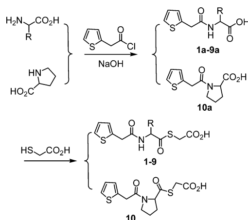
Scheme 1. Synthetic Route of Mercaptoacetic Acid Thioesters
